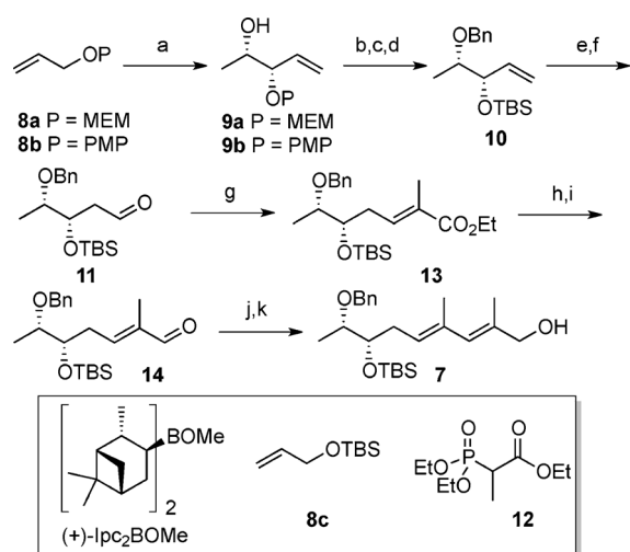
Scheme 2. a) s\text{BuLi} , THF, -78^\circ\text{C} , 30 min, then (+)-Ipc 2 BOMe, -78^\circ\text{C} , 60 min, then \text{BF}_3\cdot\text{OEt}_2 , -78^\circ\text{C} , then acetaldehyde, -78^\circ\text{C} , 3 h, then \text{H}_2\text{O}_2 , NaOH, -78^\circ\text{C} to RT, 18 h, 9a (74%, ee 93%); 9b (80%, ee 92%); b) NaH, DMF, 0^\circ\text{C} , 1 h, then BnBr, 0^\circ\text{C} to RT, 18 h, 81%; c) CAN, MeCN, \text{H}_2\text{O} , 0^\circ\text{C} , 15 min, 81%; d) TBSCl, Imidazole, DMF, RT, 18 h, 90%; e) \text{Cy}_2\text{BH} , THF, 0^\circ\text{C} , 2 h, then \text{H}_2\text{O}_2 , NaOH, 0^\circ\text{C} , 4 h, 73%; f) (\text{COCl})_2 , DMSO, \text{CH}_2\text{Cl}_2 , -78^\circ\text{C} , 1 h, then \text{NEt}_3 , -78^\circ\text{C} to RT, 1 h, 99%; g) 12 , NaH, THF, 0^\circ\text{C} , 20 min, then 11 , 0^\circ\text{C} , 2 h, 92%, E/Z = 7:1; h) DIBAL-H, Toluene, -78^\circ\text{C} , 1 h, 93%; i) \text{MnO}_2 , THF, RT, 2 h; j) 12 , NaH, THF, 0^\circ\text{C} , 20 min, then 14 , 0^\circ\text{C} , 2 h, 78%, E/Z = 4:1; k) DIBAL-H, toluene, -78^\circ\text{C} , 1 h, 59%. CAN = cerium ammonium nitrate, Cy = cyclohexyl, DIBAL-H = diisobutylaluminum hydride, DMF = N,N -dimethylformamide, DMSO = dimethylsulfoxide, Ipc = isopinocampheyl, MEM = 2-methoxyethoxymethyl, PMP = p -methoxyphenyl, TBS = tert -butyldimethylsilyl, THF = tetrahydrofuran.
