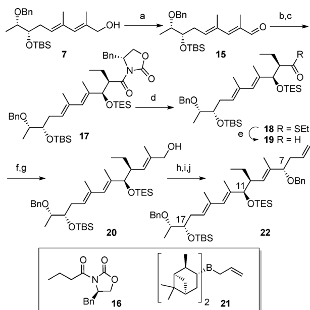
Scheme 3. a) \text{MnO}_2 , THF, RT, 2 h; b) 16 , n\text{Bu}_2\text{BOTf} , \text{NEt}_3 , \text{CH}_2\text{Cl}_2 , 0^\circ\text{C} , 30 min, then 15 , -78^\circ\text{C} to RT, then \text{H}_2\text{O}_2 , MeOH, Buffer pH 7.0, 10^\circ\text{C} to RT, 1 h, 86% over 2 steps; c) TESCl, imidazole, DMF, 0^\circ\text{C} , 20 min, 73%; d) EtSH, n\text{BuLi} , THF, 0^\circ\text{C} , 5 min, then 17 , THF, RT, 10 min, 85%; e) DIBAL-H, \text{CH}_2\text{Cl}_2 , -78^\circ\text{C} , 20 min; f) 12 , NaH, THF, 0^\circ\text{C} , 20 min, then 19 , 0^\circ\text{C} , 2 h, 70% over 2 steps, E/Z = 4:1; g) DIBAL-H, toluene, -78^\circ\text{C} , 1 h, 56%; h) \text{MnO}_2 , THF, RT, 2 h; i) 21 , THF, -78^\circ\text{C} , 1 h, then \text{H}_2\text{O}_2 , NaOH, -78^\circ\text{C} to RT, 3 h, 58%, dr = 3:1; j) NaH, n\text{Bu}_4\text{NI} , DMF, 0^\circ\text{C} , 1 h, then BnBr, 0^\circ\text{C} to RT, 18 h, 40%. TES = triethylsilyl, Tf = trifluoromethanesulfonyl.
